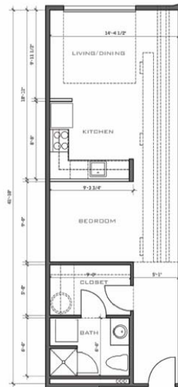
UNIT TYPE D PLAN
