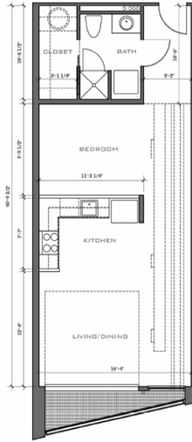
UNIT TYPE B PLAN
